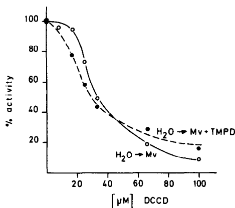
Fig.1. Effect of DCCD on the reduction of Mv with H_2O as the electron donor in the presence of NH_4Cl . The reaction mixture in 3 ml total vol. contained Tricine-NaOH, (pH 8.0) 50 mM; NaCl, 50 mM; MgCl_2 , 5 mM; Mv, 0.1 mM; NaN_3 , 0.3 mM; NH_4Cl , 10 mM; and chloroplasts equivalent to 50 \mu g chl. In the case of TMPD bypass, TMPD (30 \mu M ) and DBMIB (1 \mu M ) were added. The DCCD solution in methanol was added prior to the addition of chloroplasts. The control rates without DCCD from water to Mv and in the presence of TMPD bypass were 857 and 675 \mu equiv. \cdot \mu g \text{ chl}^{-1} \cdot h^{-1} , respectively.
