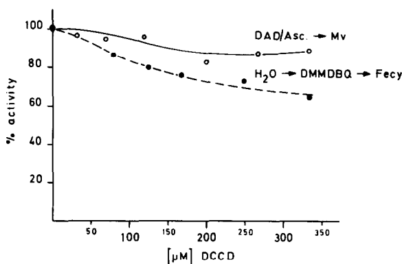
Fig.2. Effect of DCCD on the photoreduction of ferricyanide with H_2O as electron donor and Mv with DAD/ascorbate as electron donor. The reaction mixture as in fig.1 contained either: ferricyanide, 3 mM; DMMDBQ, 0.4 mM; DBMIB, 1 \mu M ; or Mv, 0.1 mM; NaN_3 , 0.3 mM; DAD, 1 mM; ascorbate, 3 mM; DCMU, 1 \mu M . The control rates in the absence of DCCD were 390 \mu equiv. and 1740 \mu equiv. for ferricyanide and Mv reduction, respectively. NH_4Cl did not improve the rates of either reaction.
